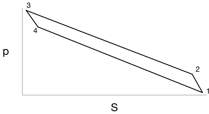
p-S Diagram
